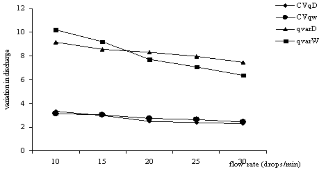
Fig 1: Effect of flow rate on discharge
