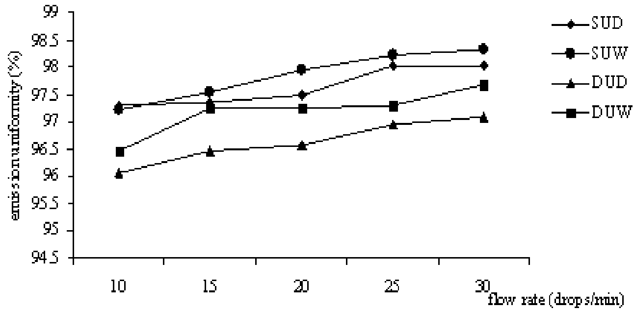
Fig 2: Effect of flow rate on emission uniformity
